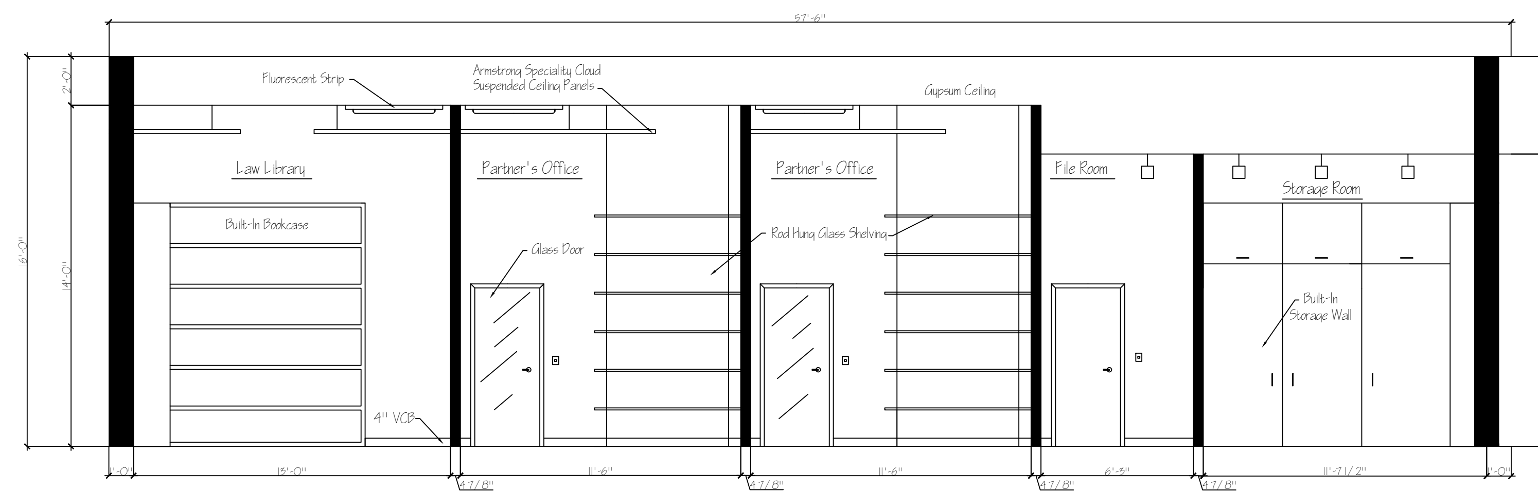
B TRANSVERSE SECTION SCALE: 1/4" = 1'-0"
